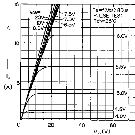
Typical Output Characteristic
