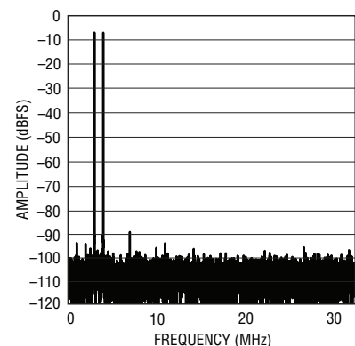
LTC2258-12 2-Tone FFT, f IN = 68MHz and 69MHz
