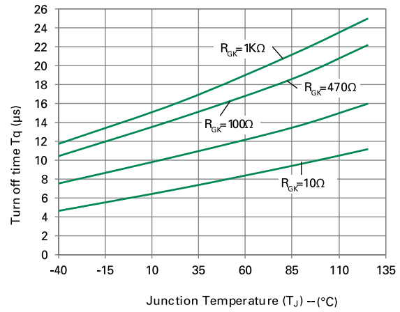
Figure 10-2: Typical DC turn off time with R_{GK} vs. Junction Temperature for S8X8ESRP
