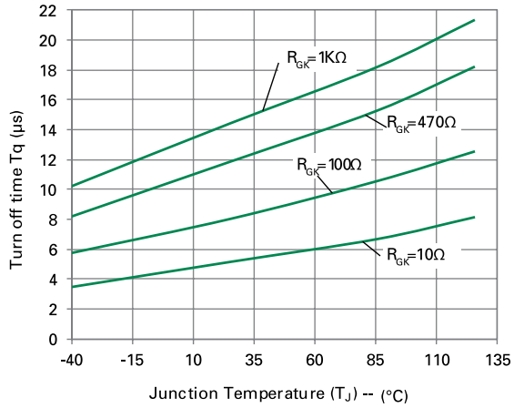
Figure 10-1: Typical DC turn off time with R_{GK} vs. Junction Temperature for S6X8BS
