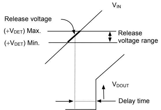
Figure 30 Release Voltage
