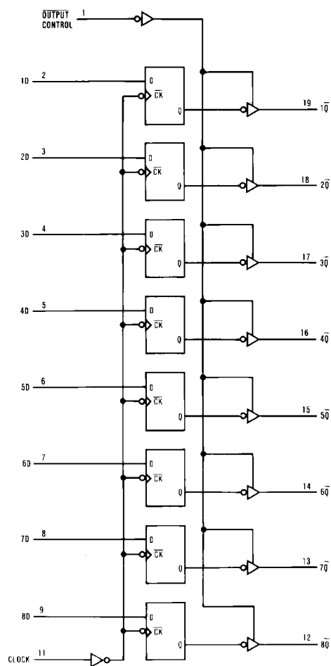
Logic Diagram
