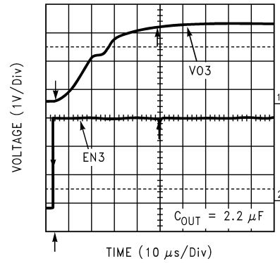
LDO3 Enable Response ( C_{OUT}=2.2\mu F )
