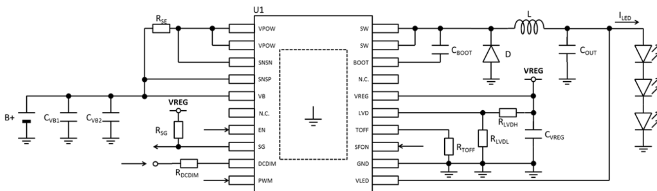
Figure 34. V_B = 13\text{ V} , I_{LED} = 2\text{ A} , LED = 3 Series, Frequency = 210 kHz
