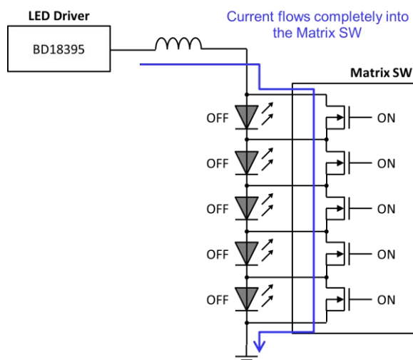
Figure 6. Current Path at Zero LED
