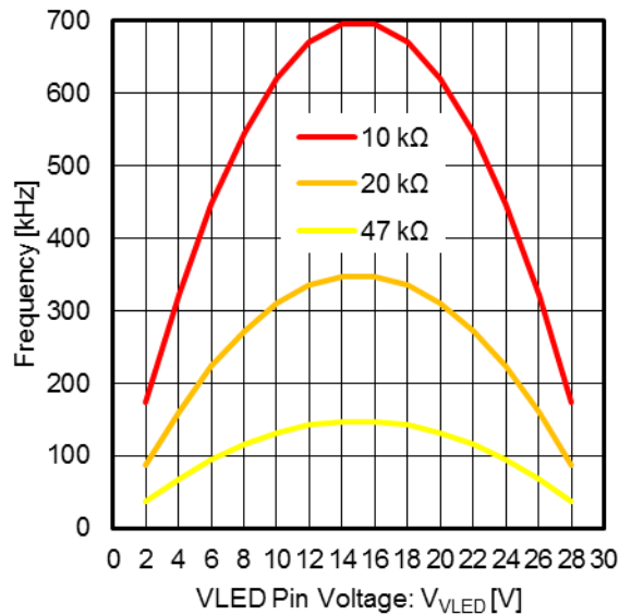
Figure 3. Switching Frequency vs V_{LED} (V_{SNSP} = 30 \text{ V}, V_{SBD} = 0.7 \text{ V}, R_{TOFF} = 10 \text{ k}\Omega, 20 \text{ k}\Omega, 47 \text{ k}\Omega)
