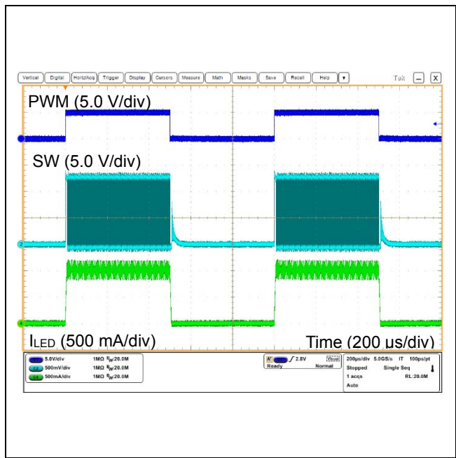
Figure 29. PWM Dimming (V B = 13 V, V SNRP = 13 V, L = 47 μH, I LED = 1 A, PWM = 1 kHz, Duty = 50 %)
