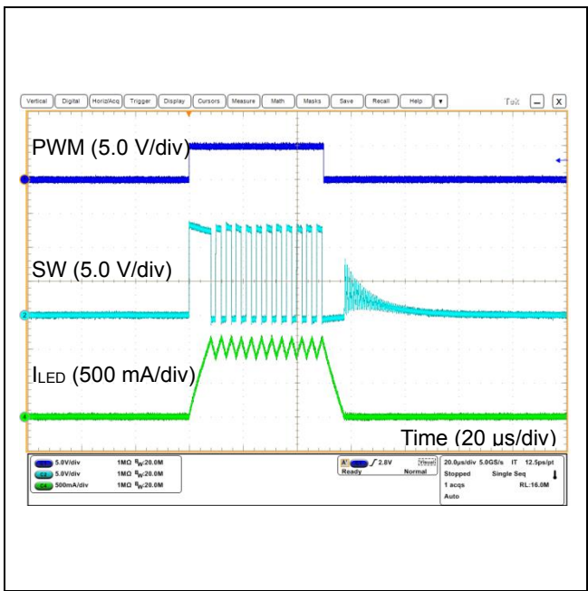
Figure 30. PWM Dimming (V B = 13 V, V SNRP = 13 V, L = 47 μH, I LED = 1 A, PWM = 1 kHz, Duty = 0.5 %)
