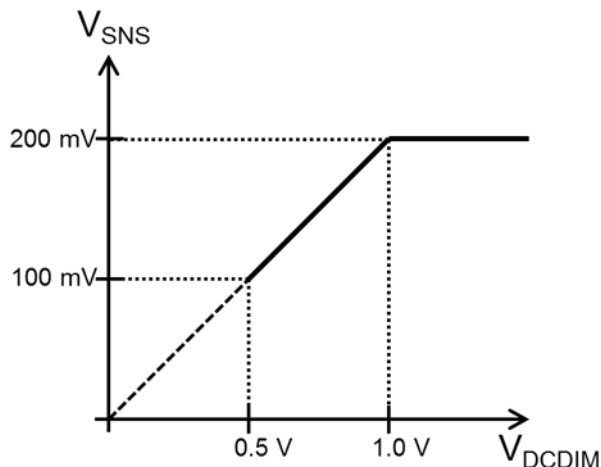
Figure 5. Analog Dimming
