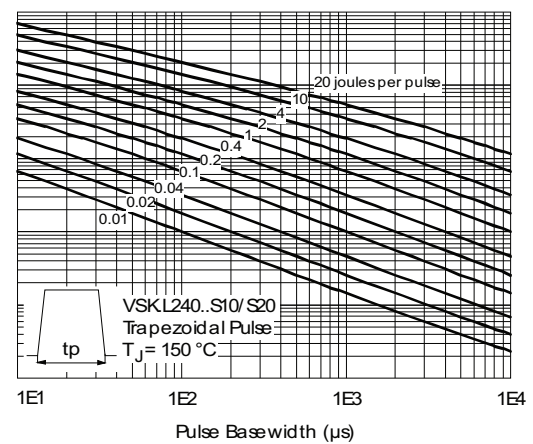
Fig. 21 - Maximum Forward Energy Power Loss Characteristics
