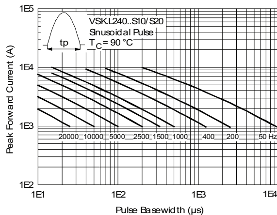
Fig. 22 - Frequency Characteristics
