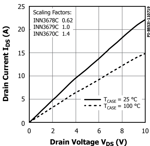
Figure 35. Output Characteristics.
