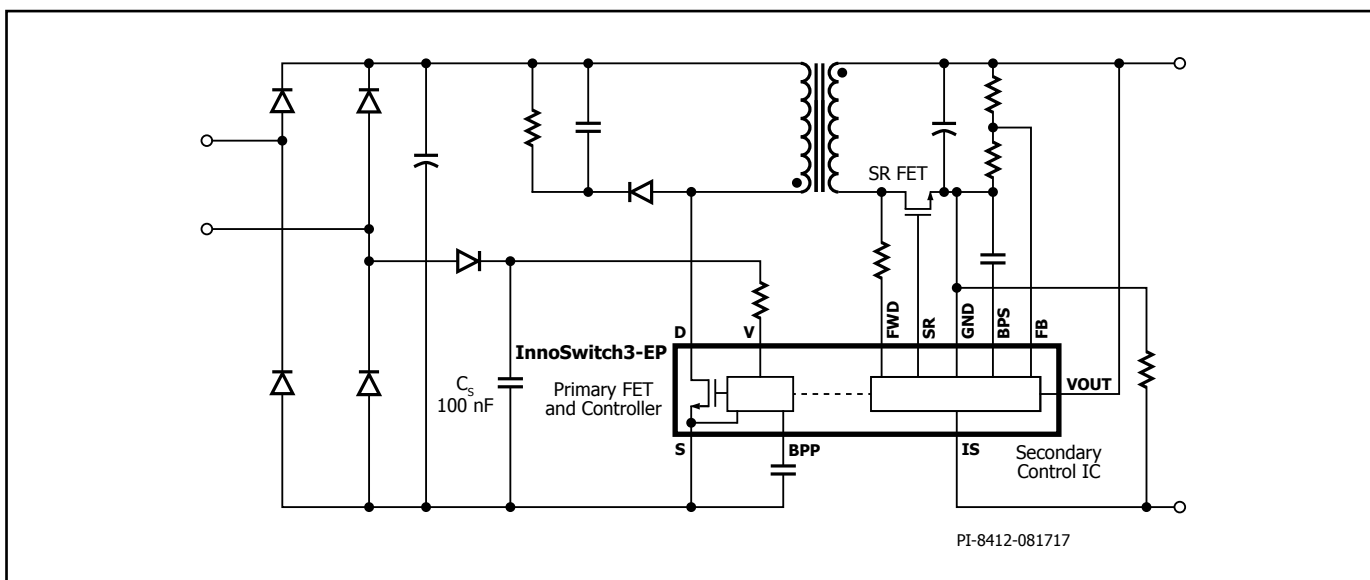
Figure 18. Fast AC Reset Configuration.
