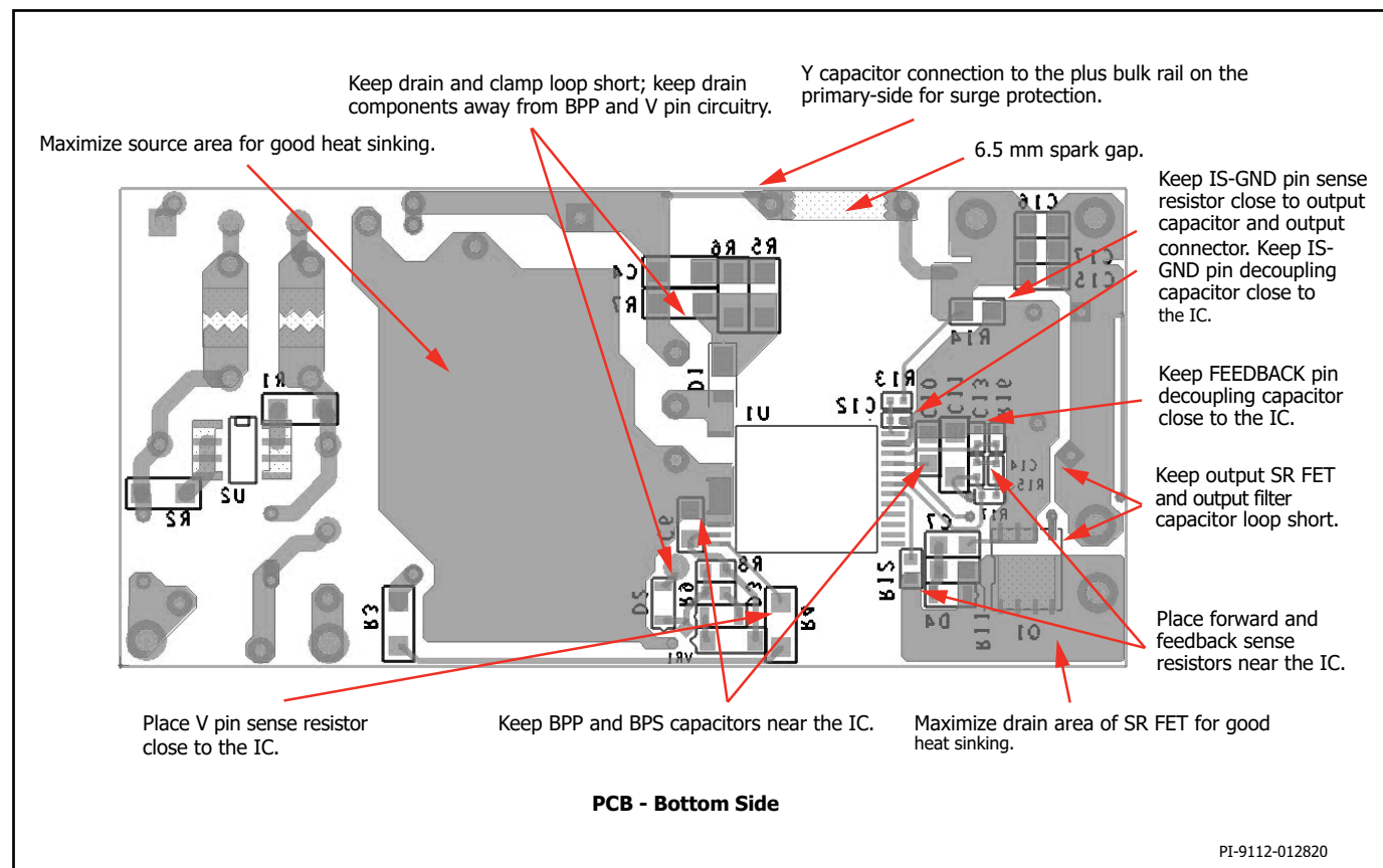
Figure 12. PCB Layout.
