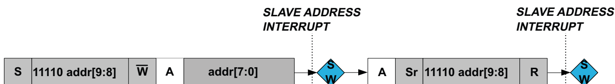
Figure 26-12.10-bit Addressing
