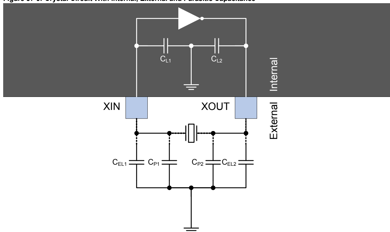
Figure 37-9. Crystal Circuit With Internal, External and Parasitic Capacitance
