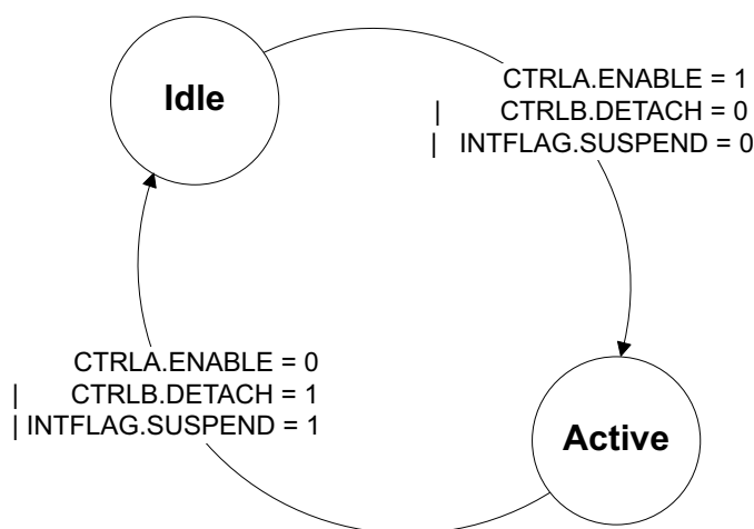
Figure 30-11. Pad Behavior
