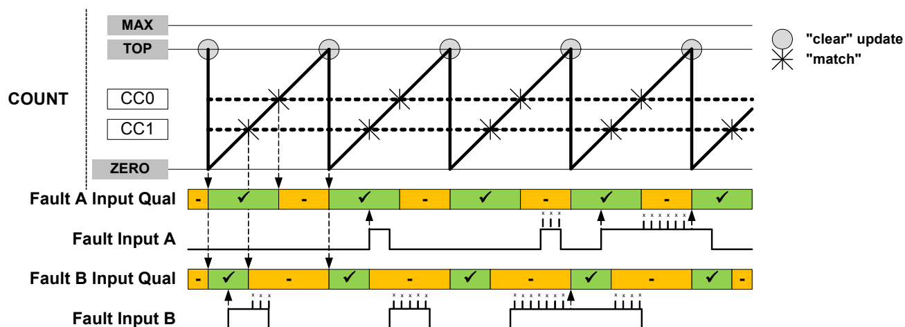
Figure 29-22. Fault Qualification in RAMP1 Operation
