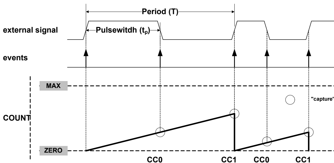
Figure 29-16. PWP Capture
