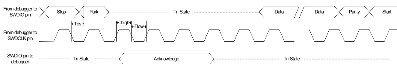
Figure 35-15.SWD Interface Signals
