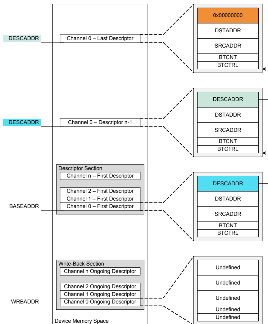
Figure 18-9. Descriptor initialization.
