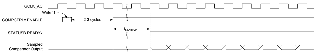
Figure 32-2. Continuous Measurement Example
