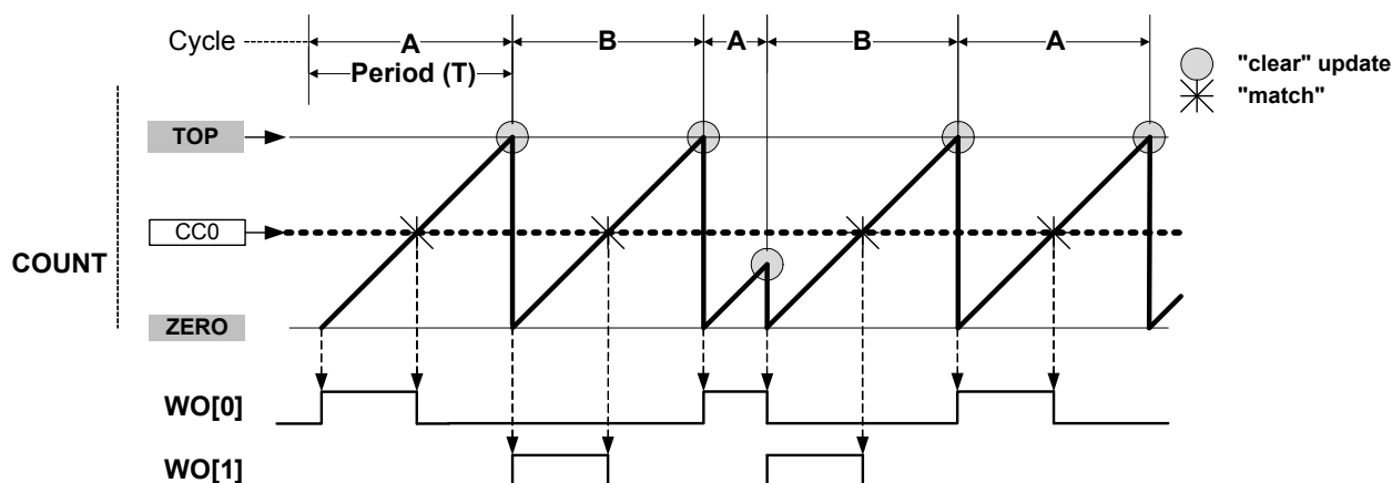
Figure 29-19.RAMP2 Alternate Operation
