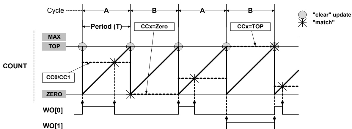
Figure 29-18.RAMP2 Operation
