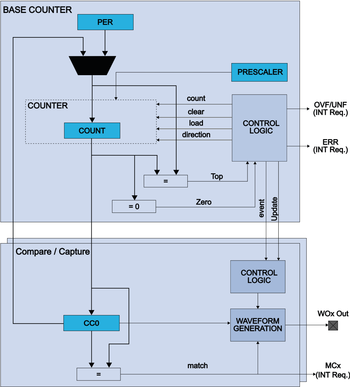
Figure 28-1. Timer/Counter Block Diagram
