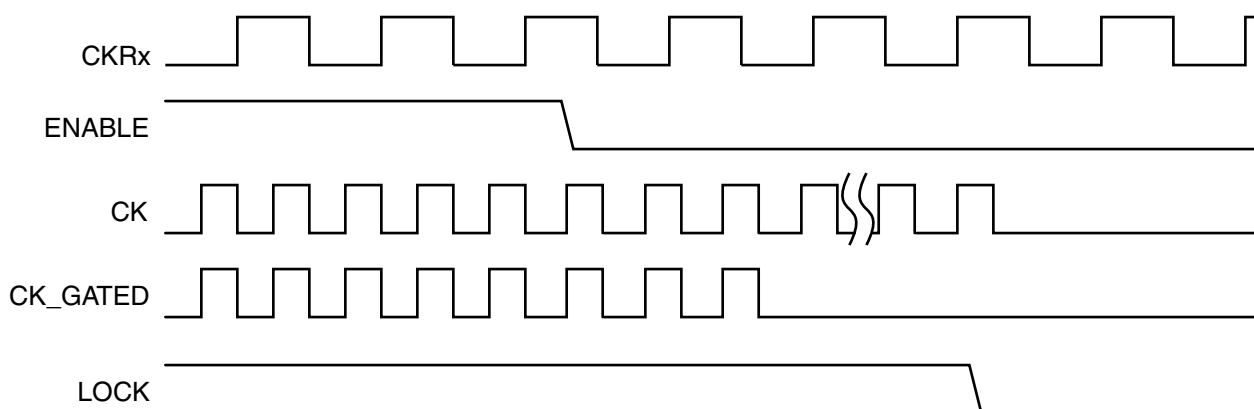
Figure 15-5. CK and CK_GATED Output from Running Mode to FDPLL96M Off Mode
