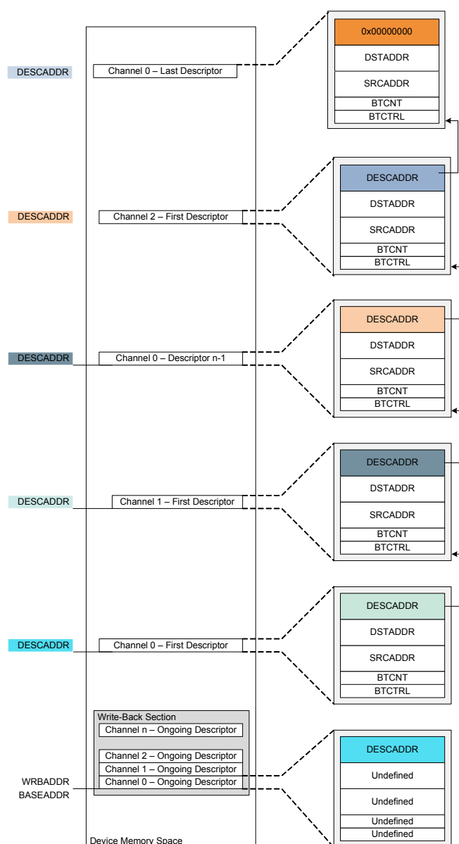
Figure 18-8. Descriptor initialization.
