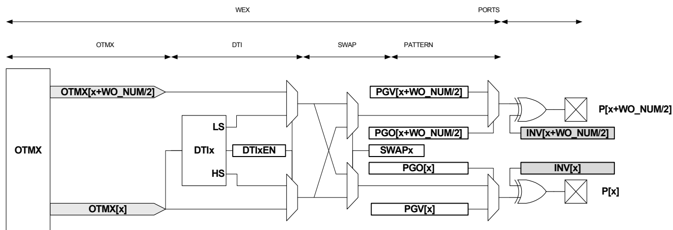
Figure 29-32.WEX Stage Details
