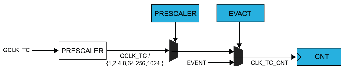
Figure 28-2. Prescaler
