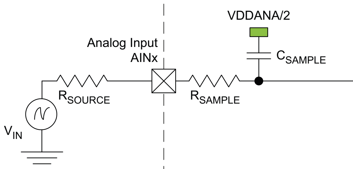
Figure 35-3. ADC Input
