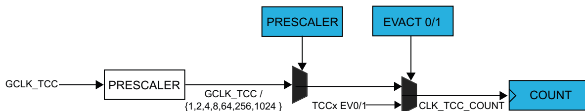
Figure 29-2. Prescaler
