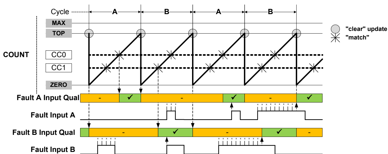
Figure 29-23. Fault Qualification in RAMP2 Operation with Inverted Polarity
