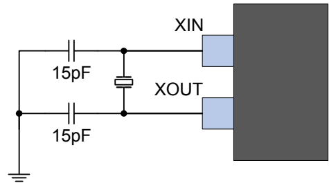
Figure 37-6. Crystal Oscillator Example Schematic
