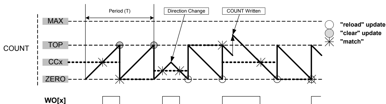
Figure 29-4. Normal Frequency Operation
