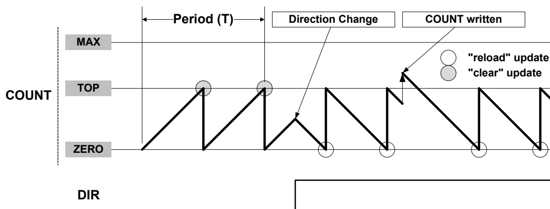
Figure 29-3. Counter Operation
