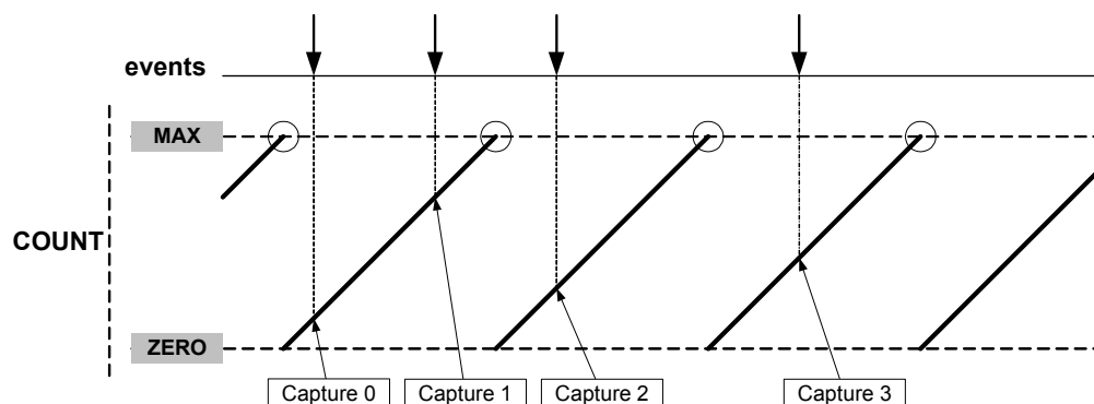
Figure 29-14.Input Capture Timing
