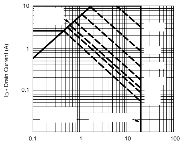
> minimum V GS at which R DS(on) is specified Safe Operating Area, Junction-to-Ambient
