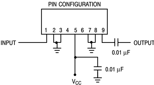
Figure 1. External Connections
