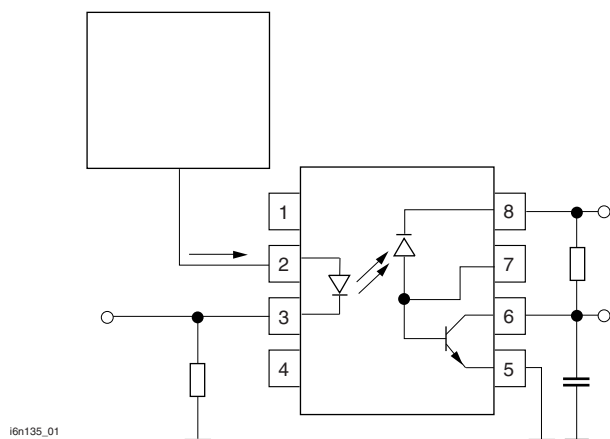
Fig. 10 - Switching Times
