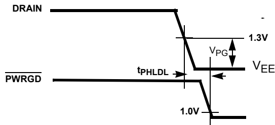
FIGURE 4A. DRAIN TO PWRGD TIMING (ISL6141)
