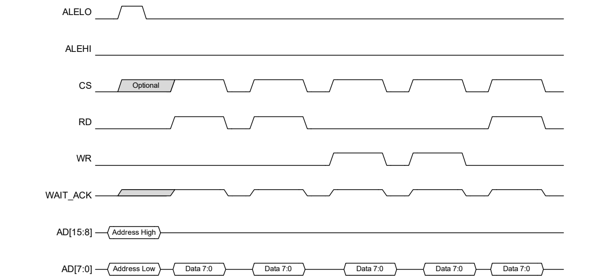
FIGURE 8-19: MULTIPLEXED ADDRESSING WITH SINGLE PHASE LATCHING - 8-BIT READS AND WRITES CONSTANT ADDRESS
