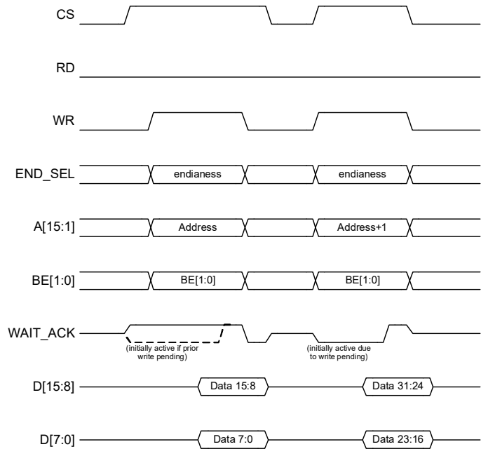
FIGURE 8-51: DEMULTIPLEXED ADDRESSING - 16-BIT POSTED WRITE
