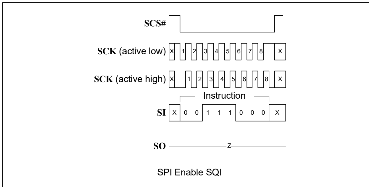
FIGURE 9-3: ENABLE Sqi
