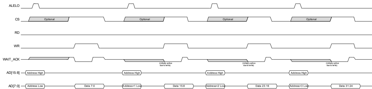
FIGURE 8-49: MULTIPLYED ADDRESSING WITH SINGLE PHASE LATCHING - 8-BIT NON-POSTED WRITE
