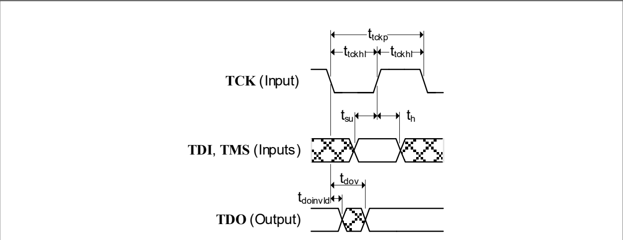
FIGURE 16-1: JTAG TIMING
