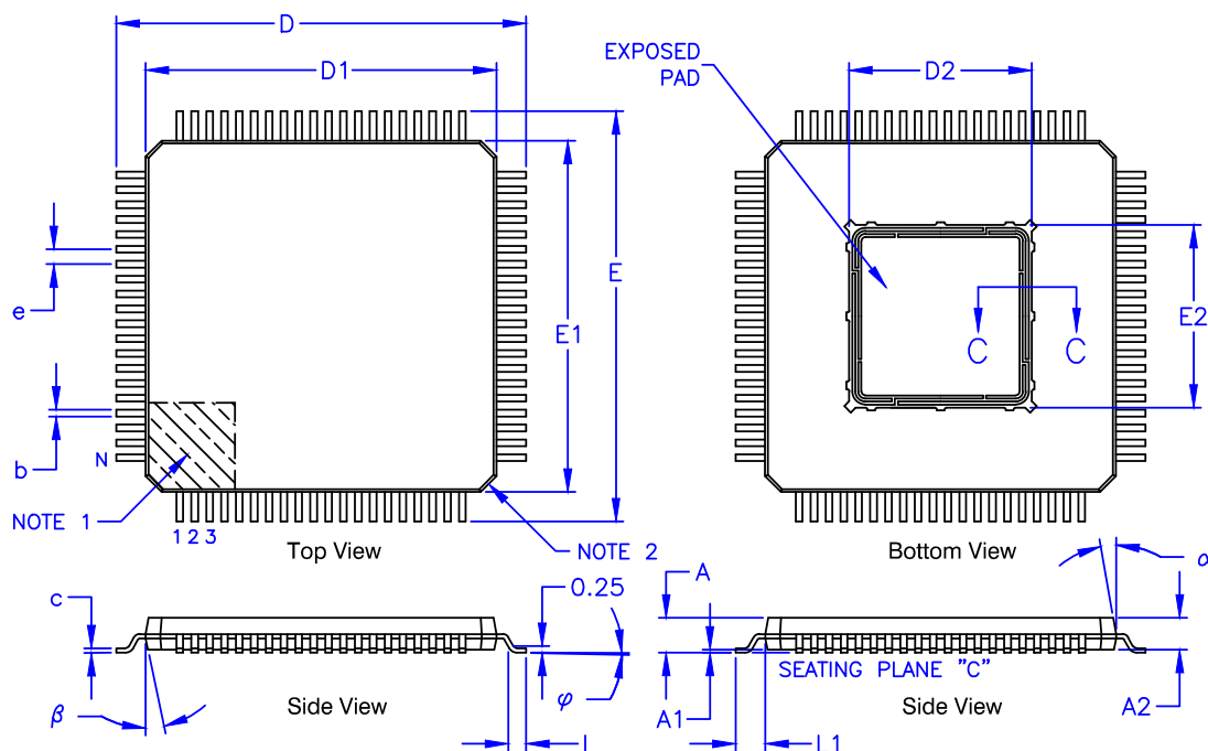
FIGURE 18-1: 80-TQFP-EP PACKAGE
