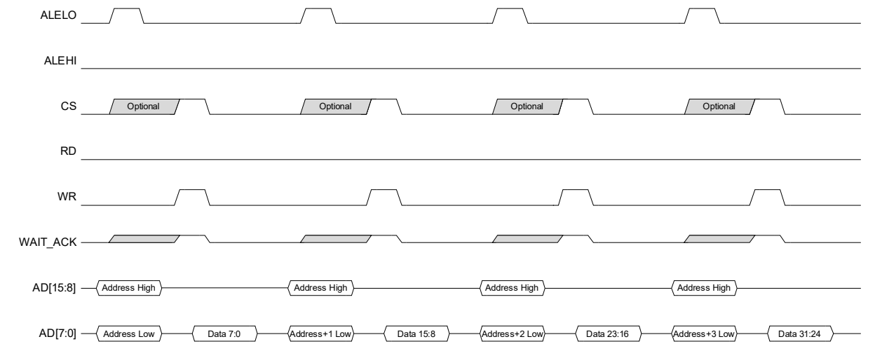
FIGURE 8-18: MULTIPLEXED ADDRESSING WITH SINGLE PHASE LATCHING - 8-BIT WRITE
