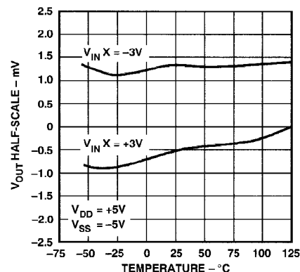
Figure 4. V_{OUT} Half-Scale ( 80_H ) vs. Temperature
