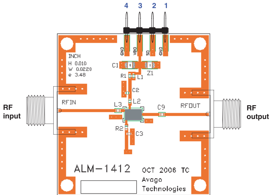
DC Pin Configuration of 4-pin Connector
