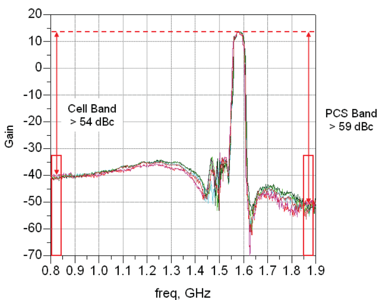
Figure 9. Multiple module plots of rejection at Cell and PCS Bands
