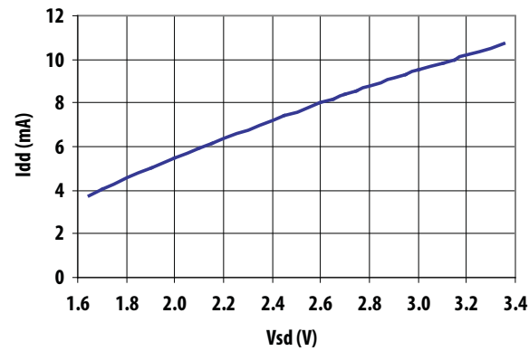
Figure 14. Idd vs. Vsd ( V_{dd} = 2.85\text{ V} )
