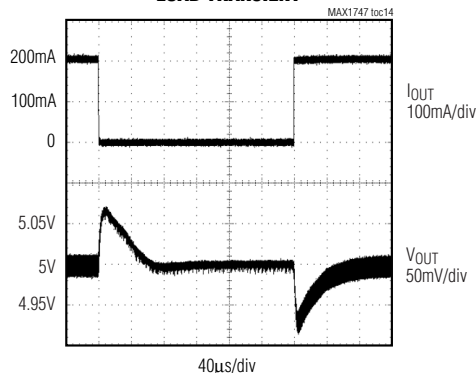
LOAD TRANSIENT
