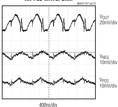
RIPPLE WAVEFORM
