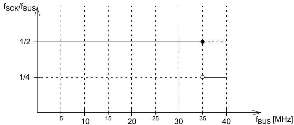
Figure 12. Derating of maximum f_{\text{SCK}} to f_{\text{BUS}} ratio in master mode
