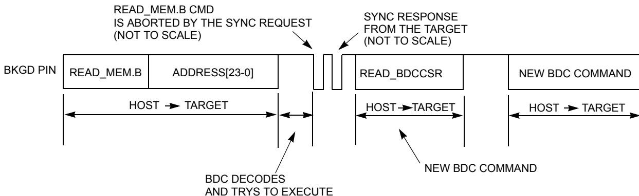
Figure 78. ACK abort procedure at the command level (not to scale)
