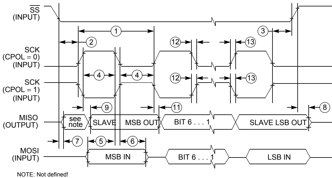
Figure 14. SPI slave timing (CPHA=1)
