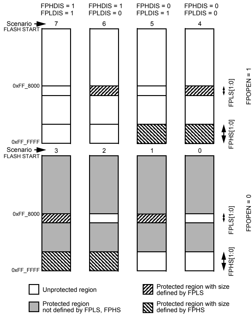
Figure 101. P-flash protection scenarios
