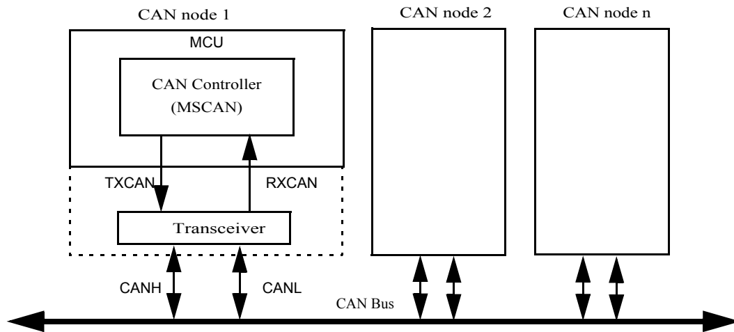
Figure 89. CAN system
