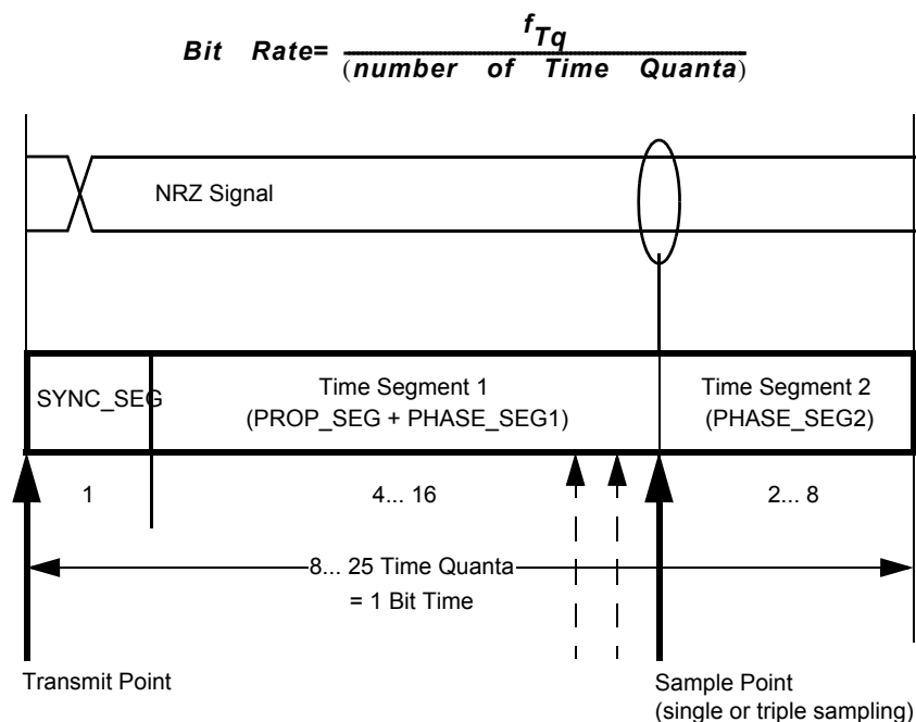
Figure 95. Segments within the bit time
