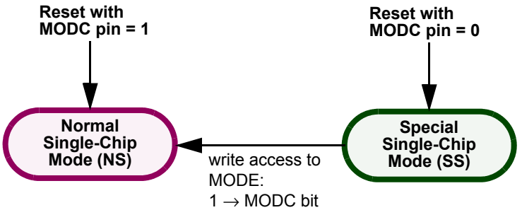
Figure 65. Mode transition diagram
