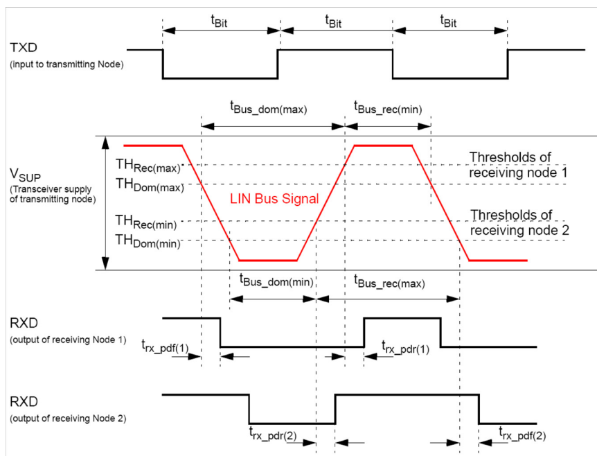
Figure 110. Definition of LIN bus timing parameters
