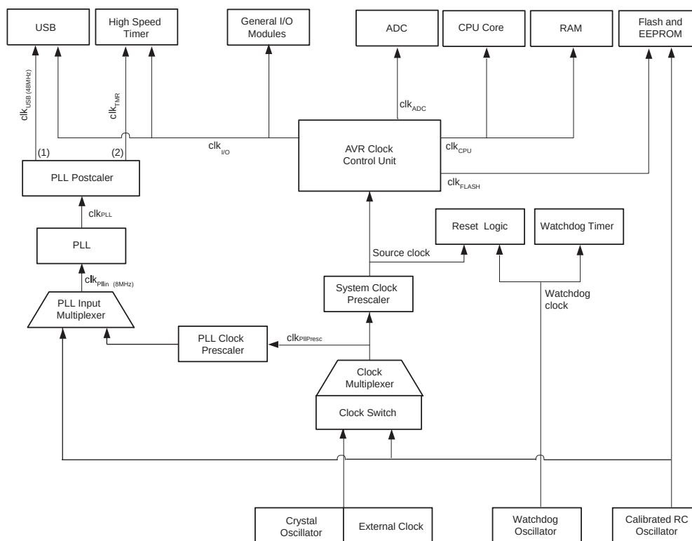
Figure 6-1. Clock Distribution
