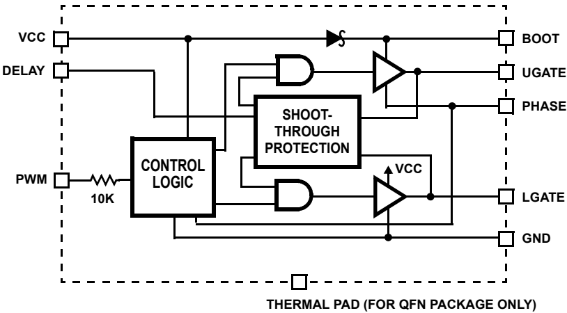
FIGURE 1. BLOCK DIAGRAM
