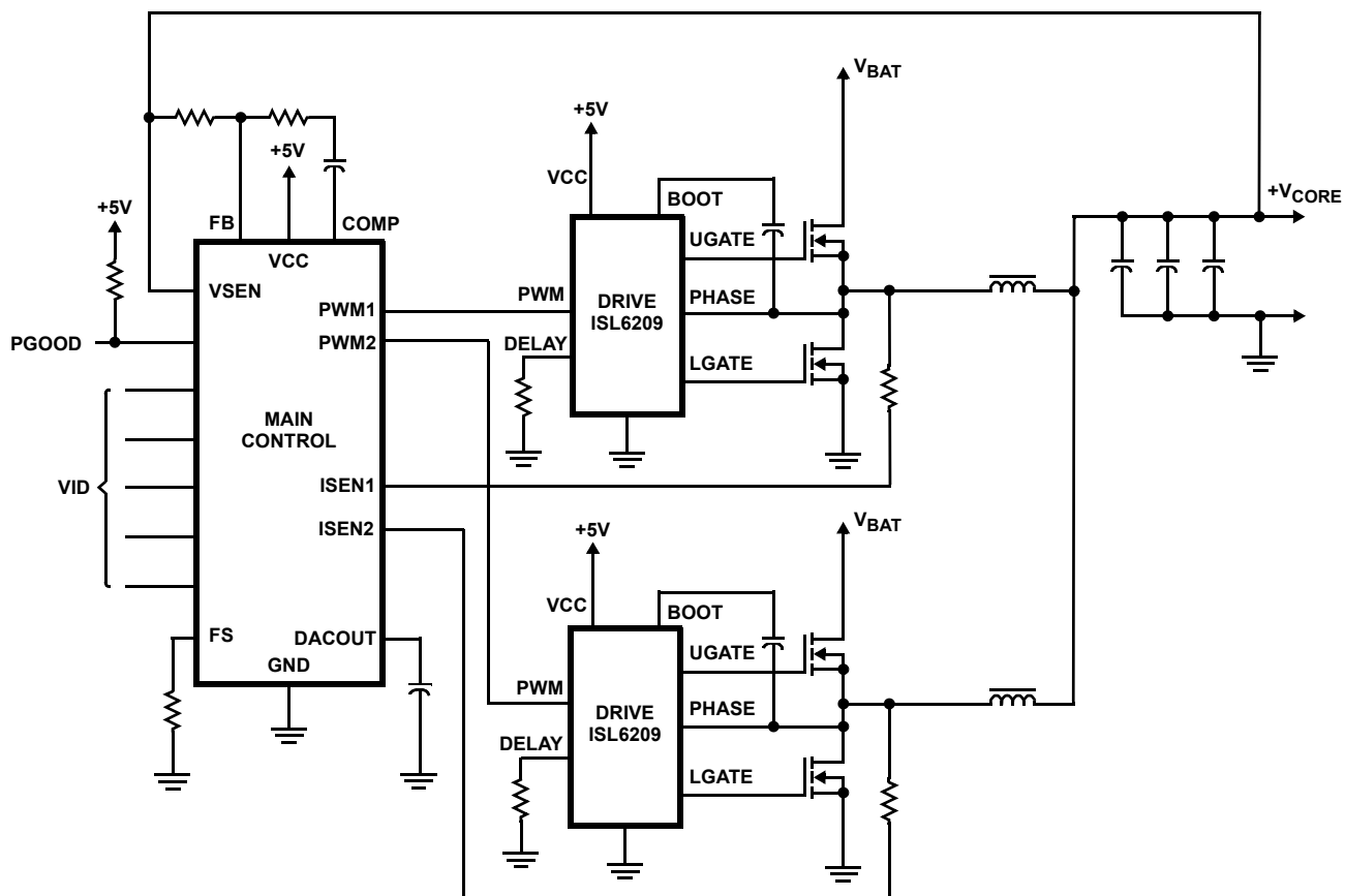
FIGURE 2. TYPICAL APPLICATION
