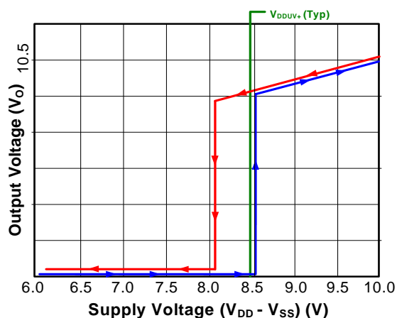
Figure 10. Si8220/21 UVLO Response (8 V)
