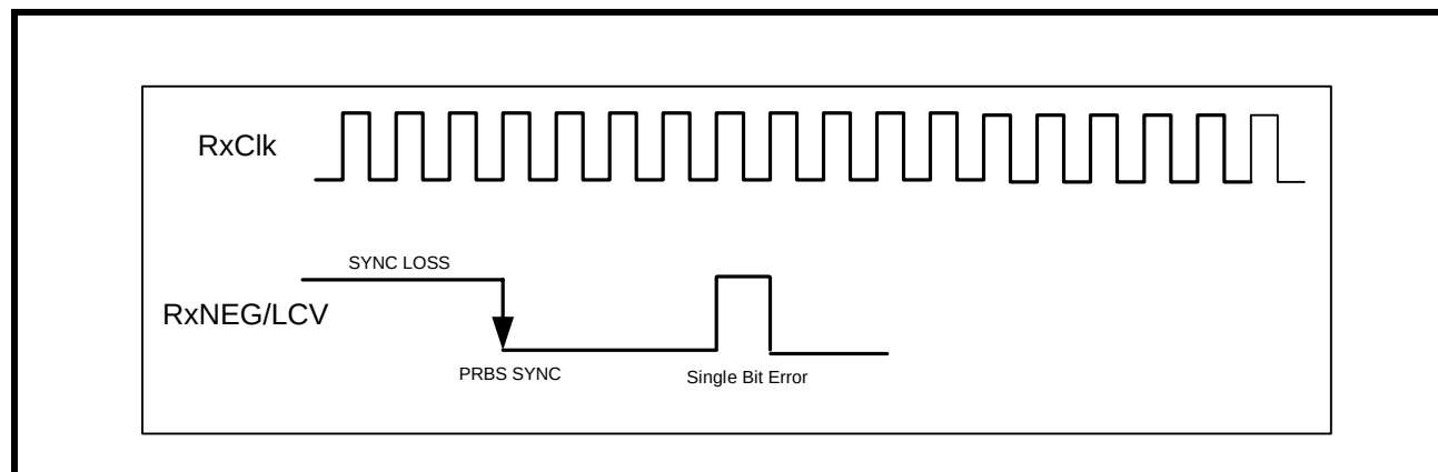
FIGURE 29. PRBS MODE
