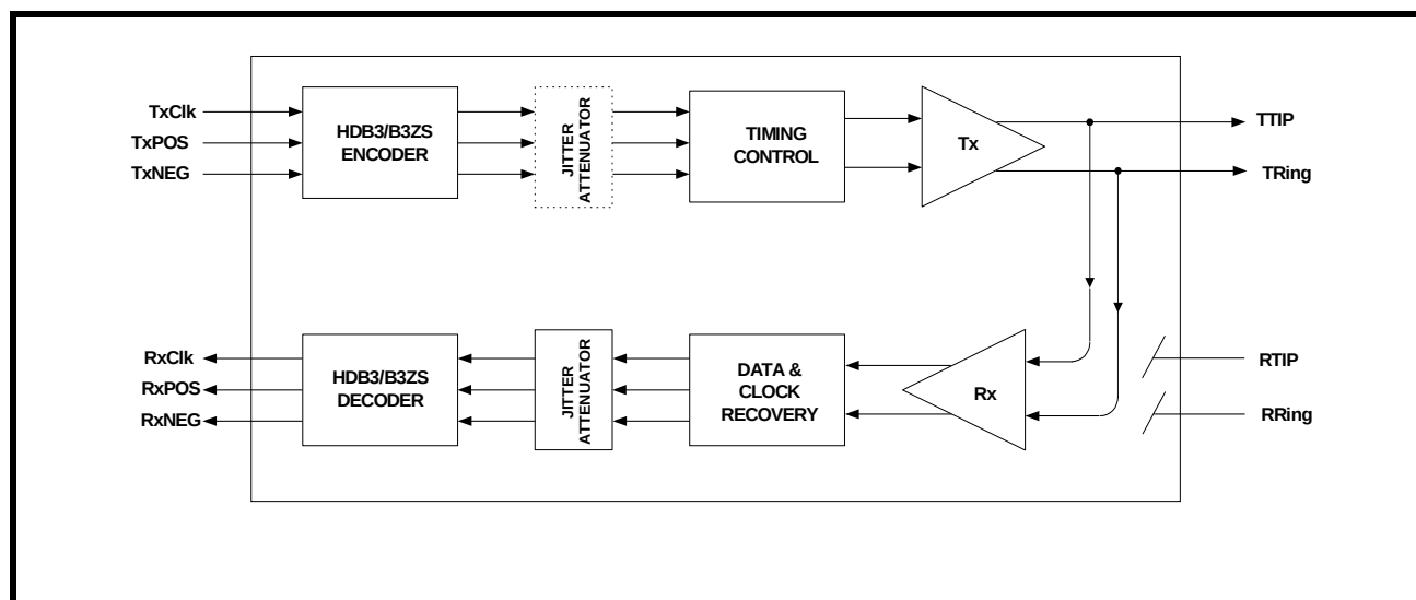
FIGURE 30. ANALOG LOOPBACK
