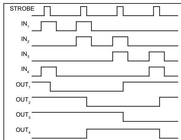
FIGURE 4-3: Unipolar 2-Phase Drive.
