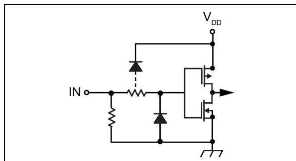
FIGURE 2-1: Typical Input.
