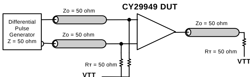
Figure 3. PECL_CLK CY29949 Test Reference for V_{CC} = 3.3 \text{ V} and V_{CC} = 2.5 \text{ V}
