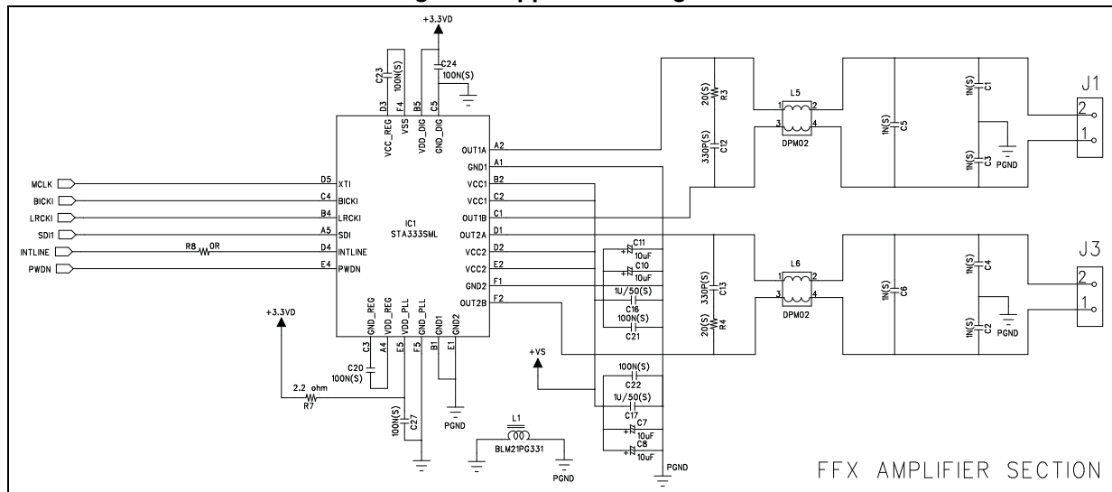
Figure 9. Application diagram
